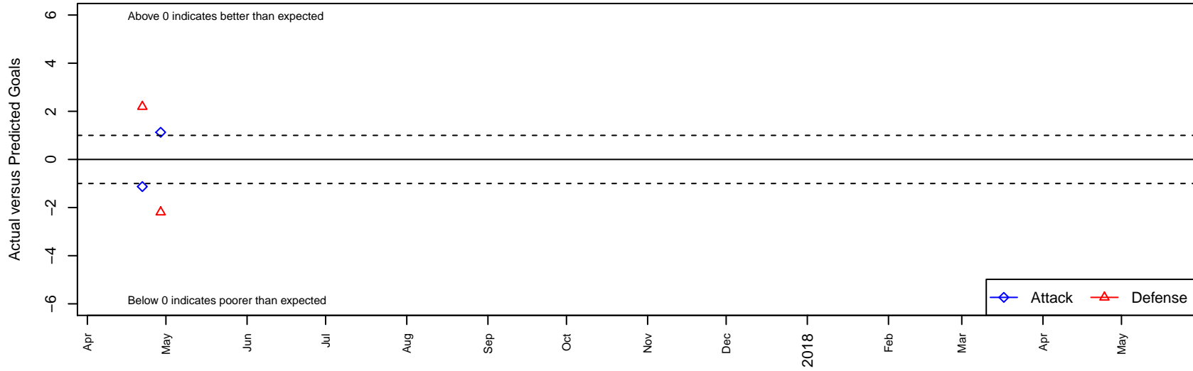
Seattle United Samba B05 Dots are actual minus expected GF (blue circles) and GA (red triangles). Blue line is smoothed change in attack strength. Red is smoothed change in defense strength.
